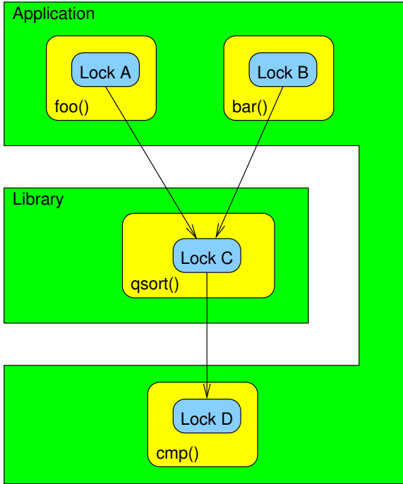
Figure 6.7: Layered Locking Hierarchy for qsort()
