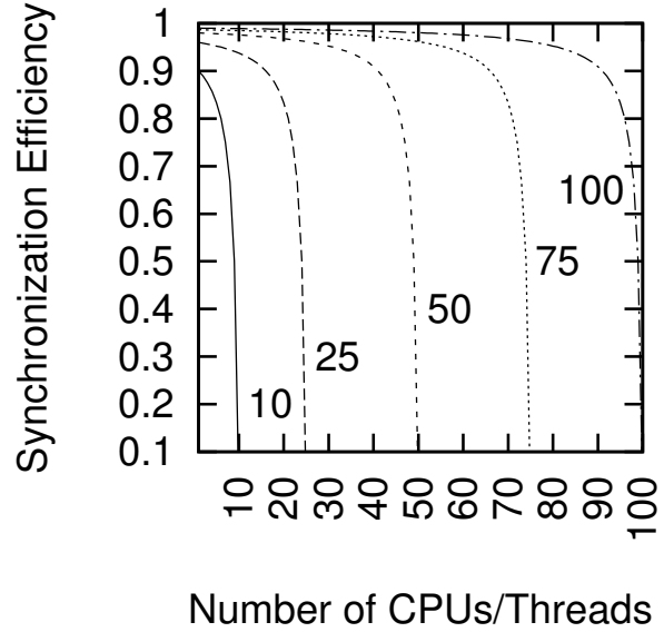
Figure 5.21: Synchronization Efficiency
